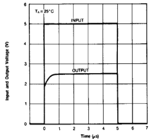
Figure 6. Pulse Response
